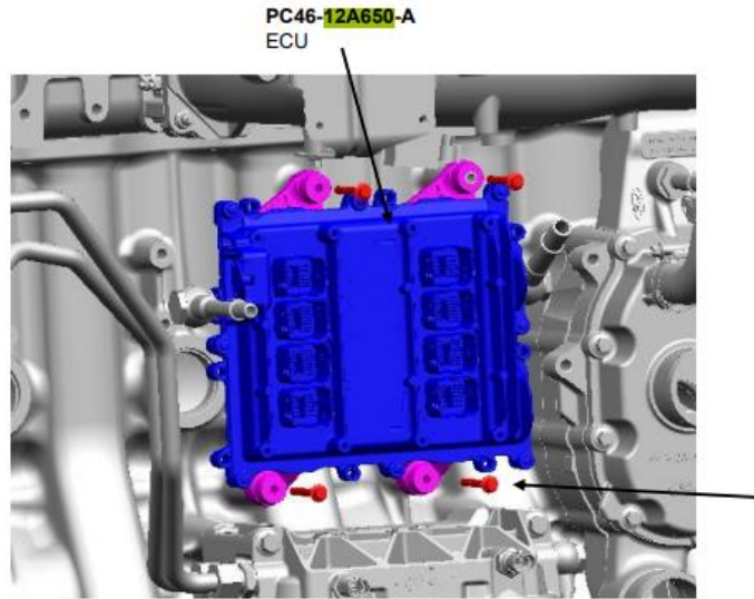
GEN 1.5 ECU LOCATION IN THE ENGINE
